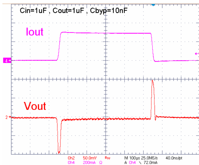
Load Transient
