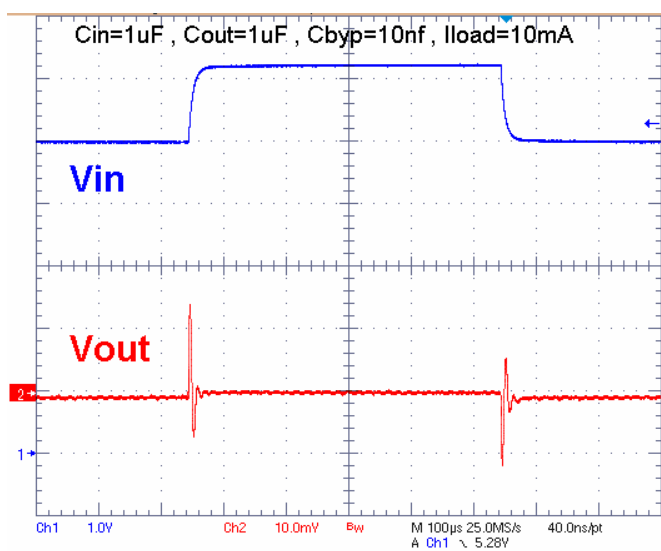
Line Transient
