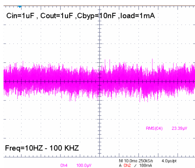
Output Voltage Noise
